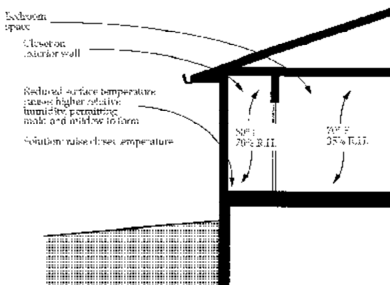
Figure 1. Closets on exterior house walls may be conducive to mold growth.
