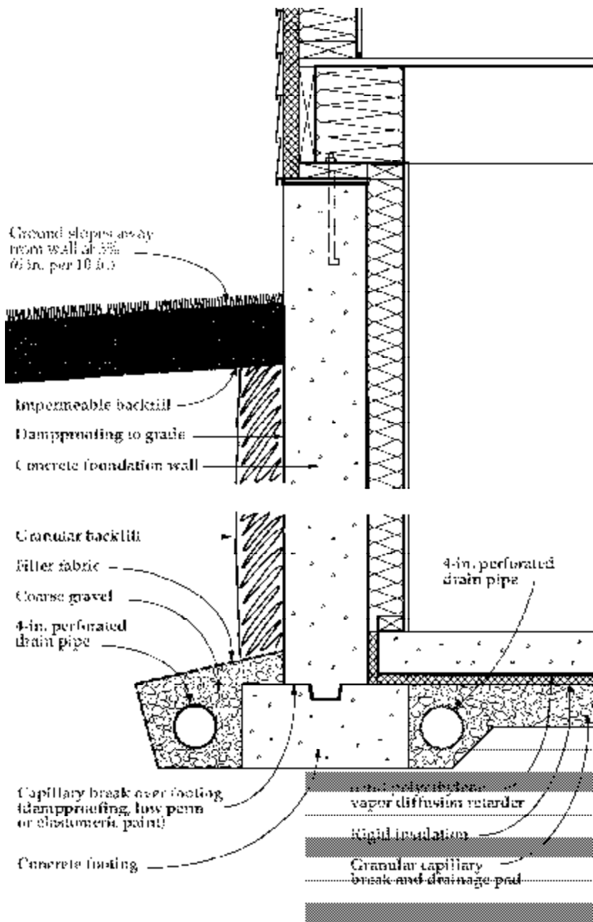
Figure 7. Foundation drainage system.
