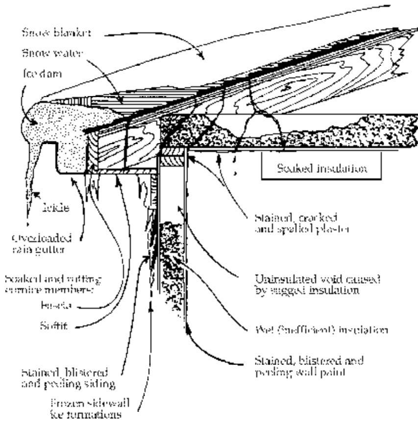
Figure 5. Problems caused by ice dams.
